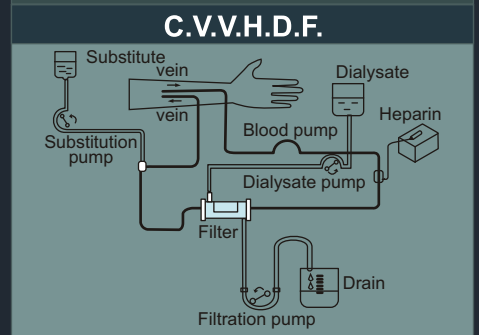
Continuous Veno - Venous Haemodiafiltration
